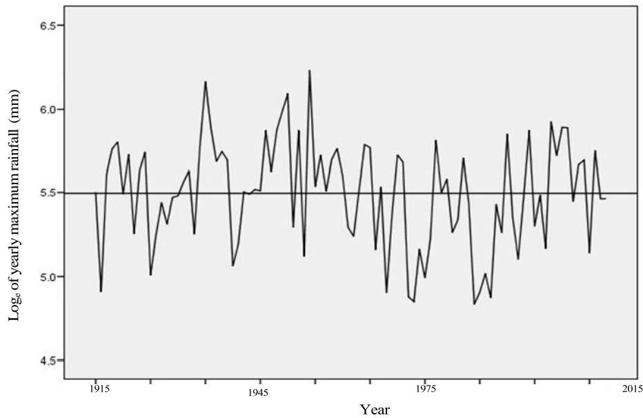
Figure 3: Sequence of yearly maximum rainfall
