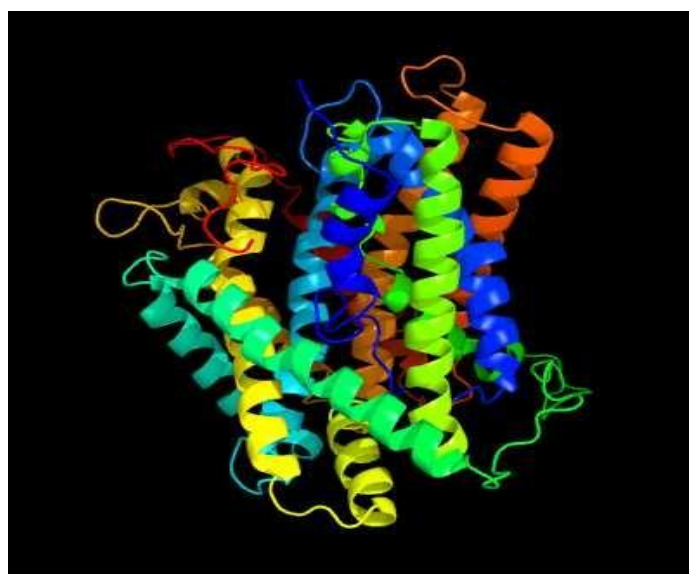
Figure 2. Schematic 3D structure of cattle amino acid permease-bovine protein Image coloured by rainbow N → C terminus Model dimensions (Å): X: 68.312 Y:64.481 Z:61.432 393 residues (97% of goat phosphoglycerate_kinase-caprine sequence) have been modelled with 100.0% confidence by the single highest scoring template.
