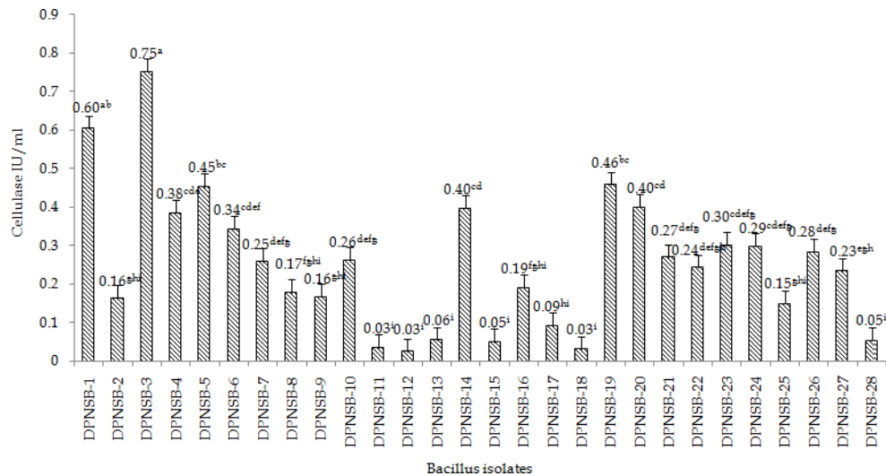
Figure 4. Production of Cellulase from Bacillus isolates
